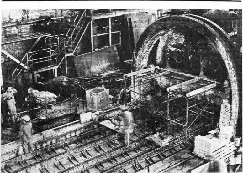
Remont v valjarni žice
