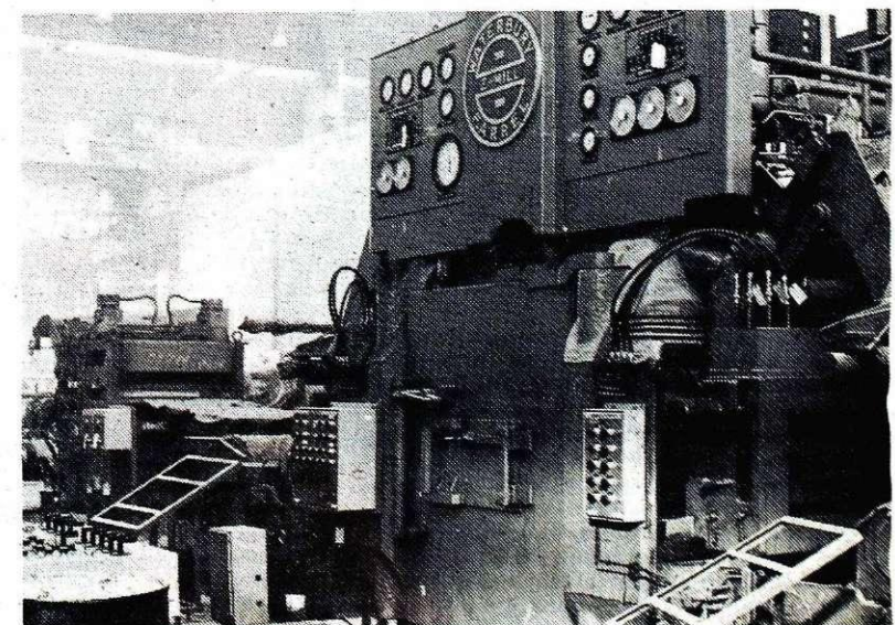
Nova hladna valjarna – sendzimir ogrodge s komandnim pultom
